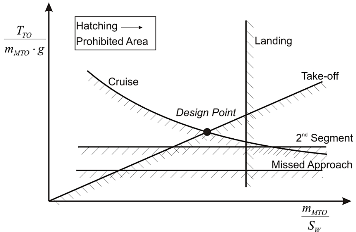
Figure 2.8 Matching chart (Scholz 2015)
