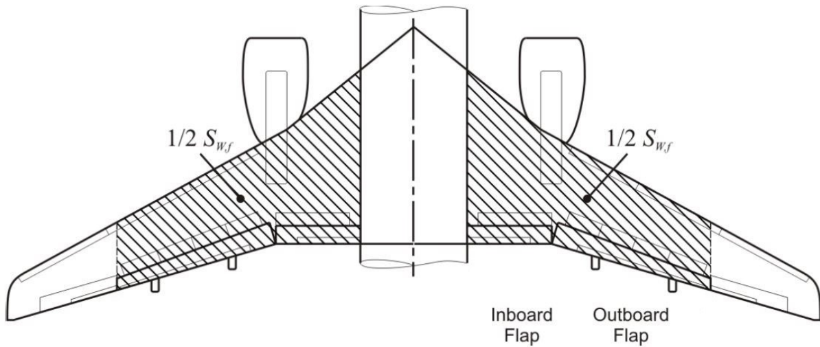
Figure 5.21 Definition of the flapped area (Scholz 2015)
