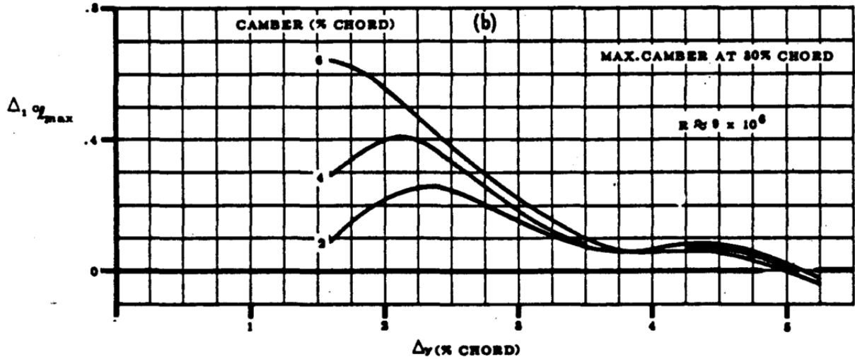
Figure 5.4 Correction term \Delta_1 c_{L,max} considering the camber and the maximum camber at 30% (DATCOM 1978)
