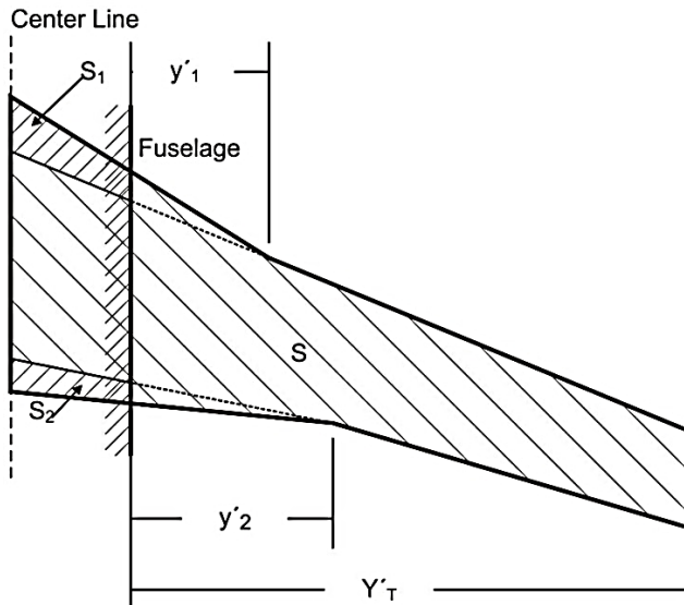
Figure 5.30 Reference area according to Boeing (Scholz 2015)
