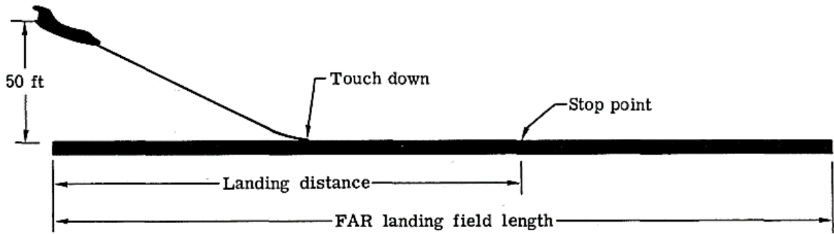
Figure 2.2 Landing field length (Loflin 1980)
