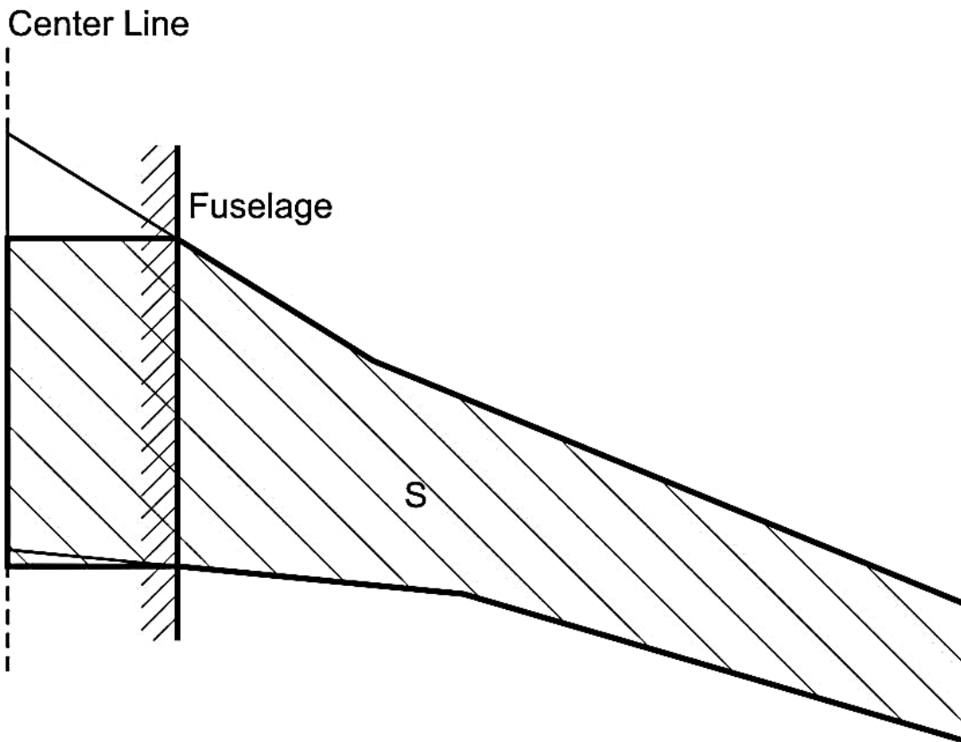
Figure 5.31 Reference area according to Airbus (Scholz 2015)
