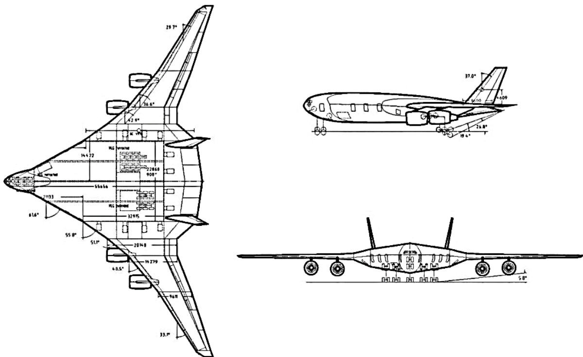
Figure 6.9 3 view drawing of the Blended Wing Body VELA 2 (Scholz 2006)
