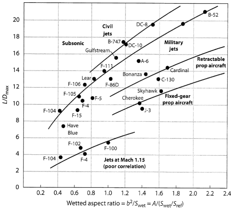
Figure 2.4 Maximum aerodynamic efficiency trends (Raymer 2012)
