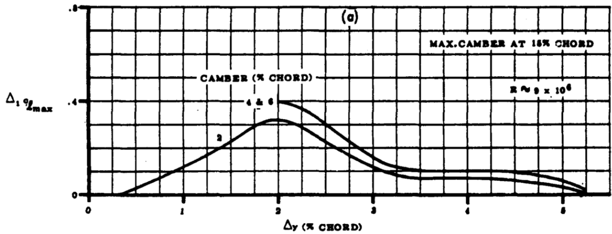
Figure 5.3 Correction term \Delta_1 c_{L,max} considering the camber and the maximum camber at 15% (DATCOM 1978)
