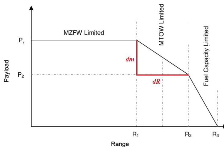
Figure 6.12 Example of a payload-range diagram. Adapted from (Haß, 2015)
